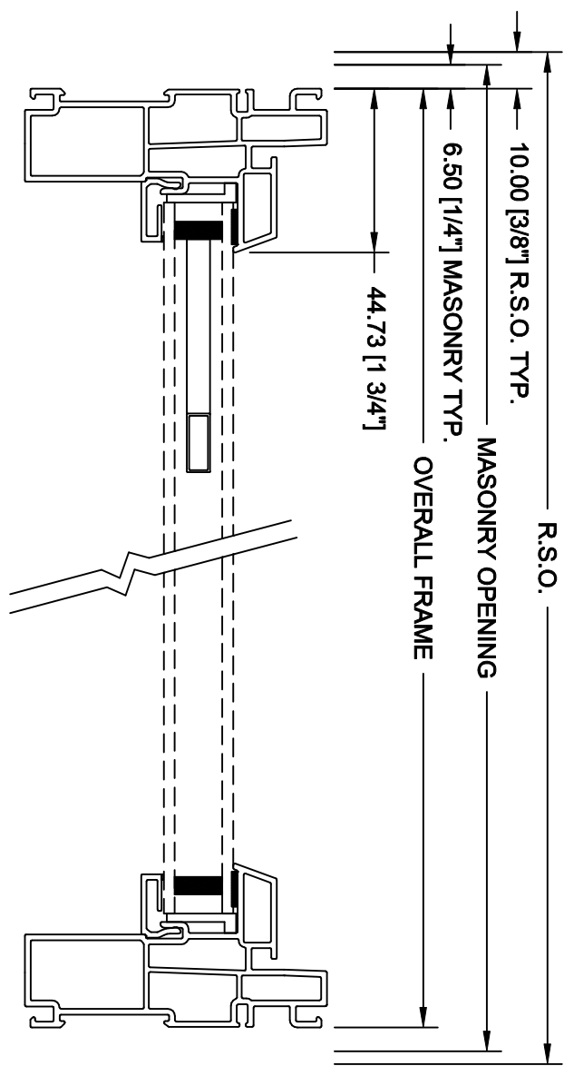
HORIZONTAL SECTION
