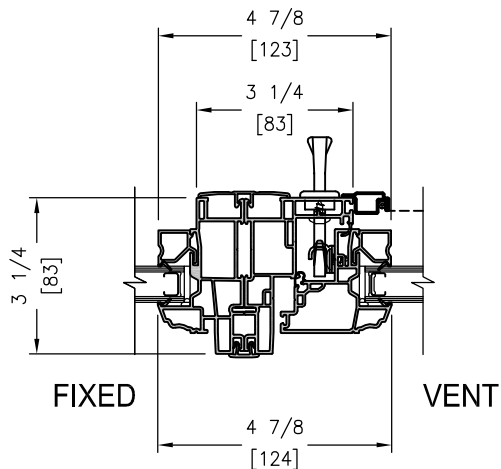
DIRECT SET TO AWNING
