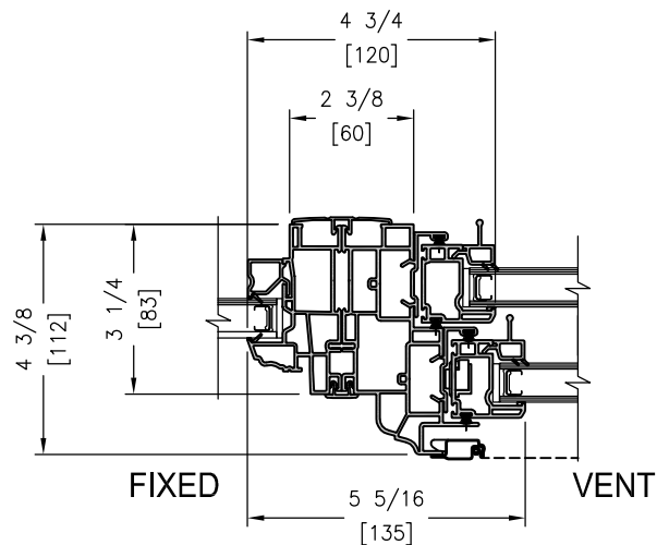
DIRECT SET TO DOUBLE SLIDER
