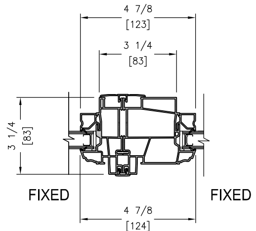
DIRECT SET TO FIXED CASEMENT
