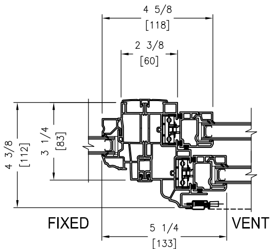
DIRECT SET TO DOUBLE HUNG
