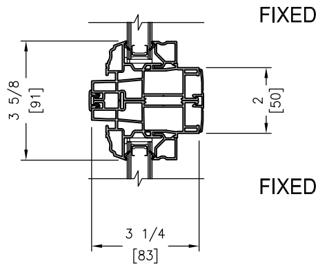
DIRECT SET OVER DIRECT SET
