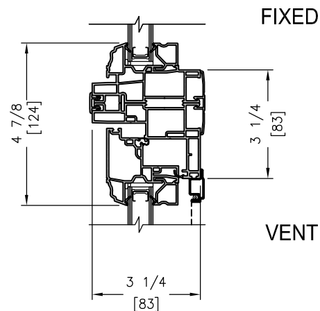
DIRECT SET OVER DOUBLE HUNG
