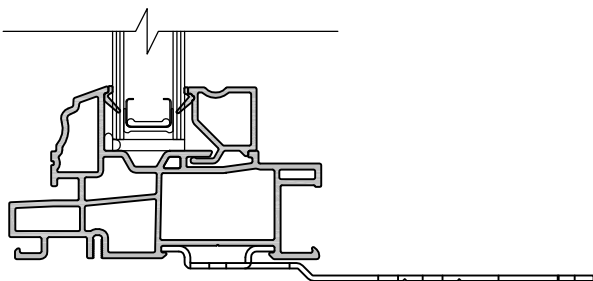
MASONRY CLIP
