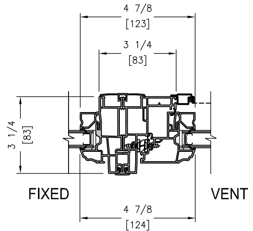
DIRECT SET OVER CASEMENT
