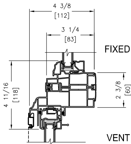
DIRECT SET OVER DOUBLE HUNG
