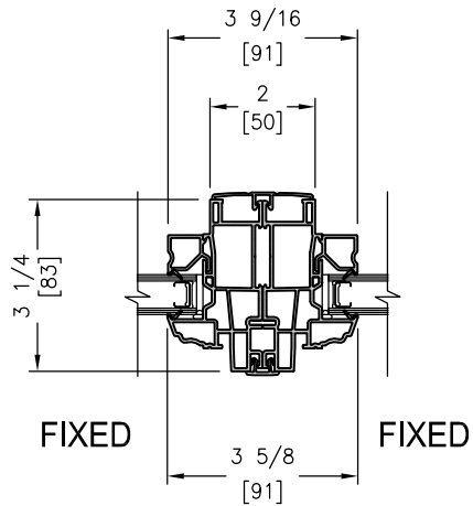
DIRECT SET TO DIRECT SET
