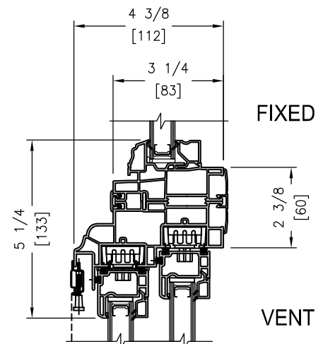
DIRECT SET OVER DOUBLE SLIDER
