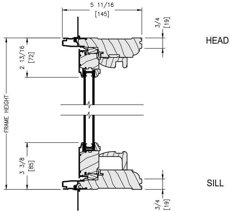
VERTICAL SECTION
