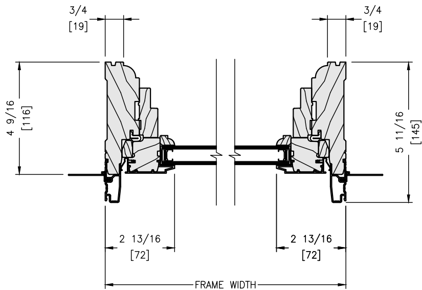
HORIZONTAL SECTION
