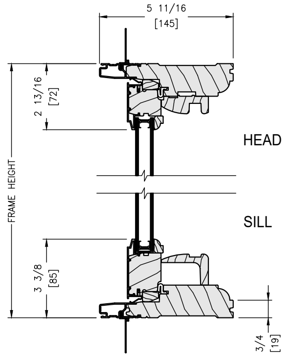
VERTICAL SECTION
