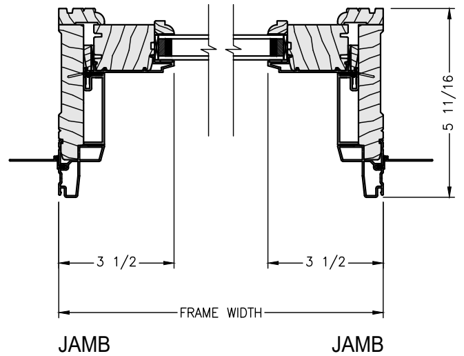
HORIZONTAL SECTION
