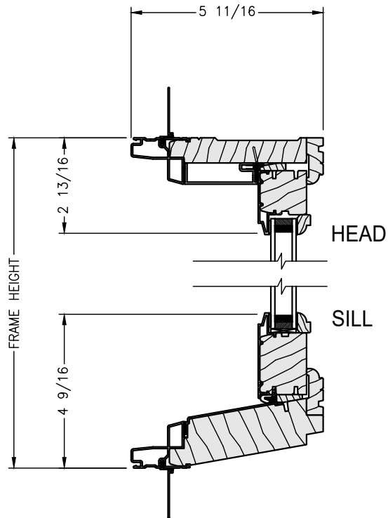
VERTICAL SECTION
