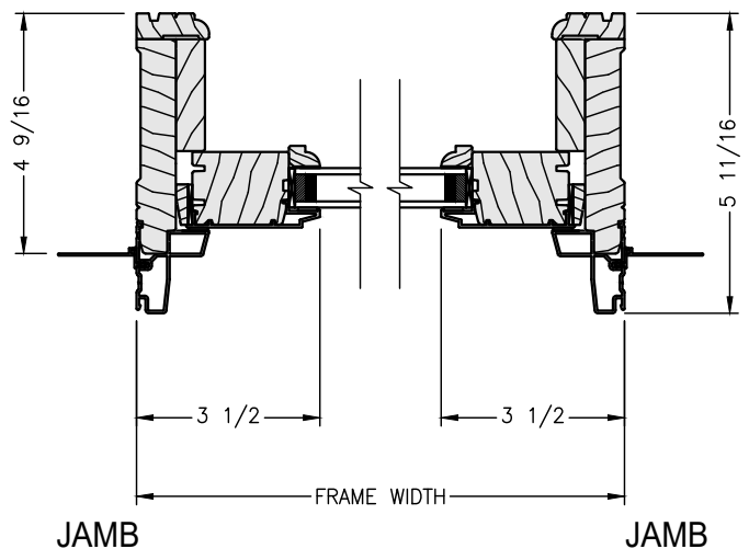
HORIZONTAL SECTION
