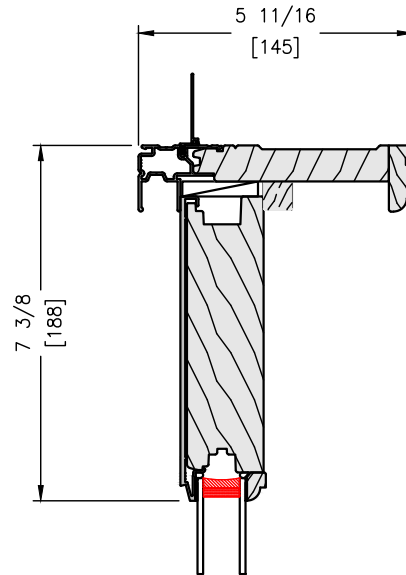
FIXED HEAD
