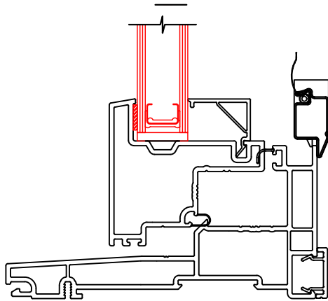
INTERIOR SLOT COVER
