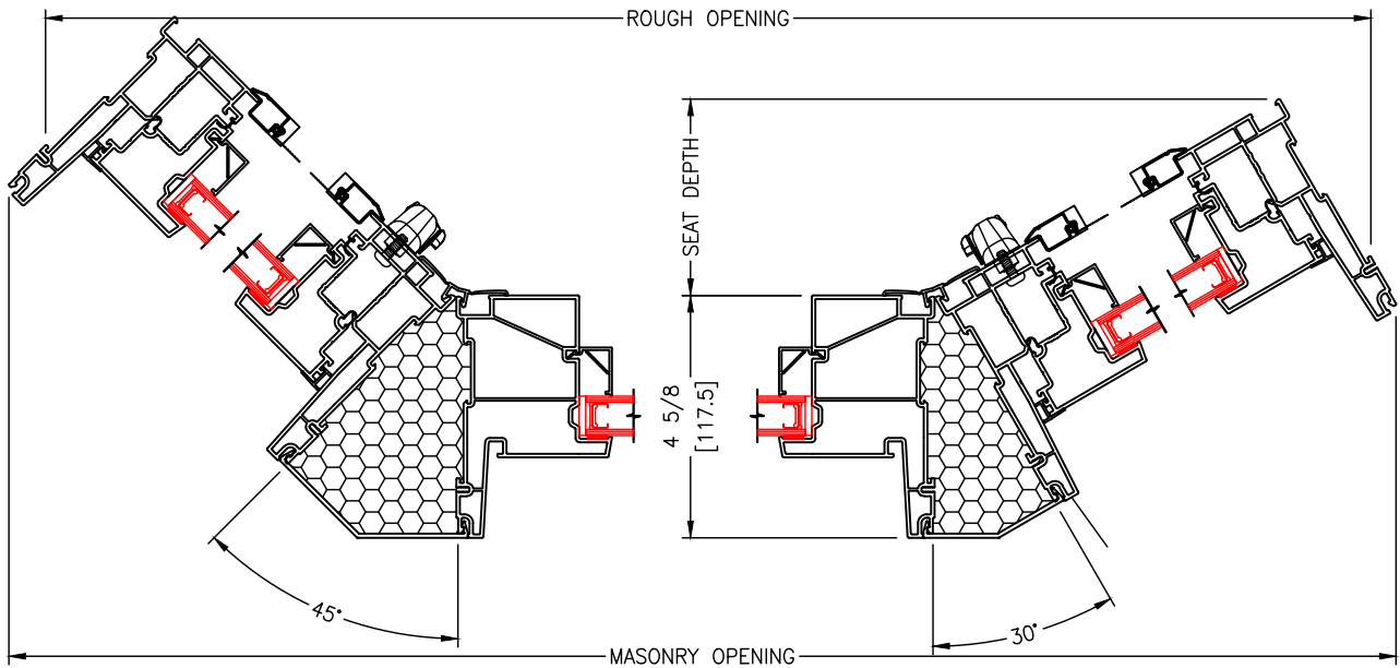
45° BAY WINDOW HORIZONTAL SECTION
