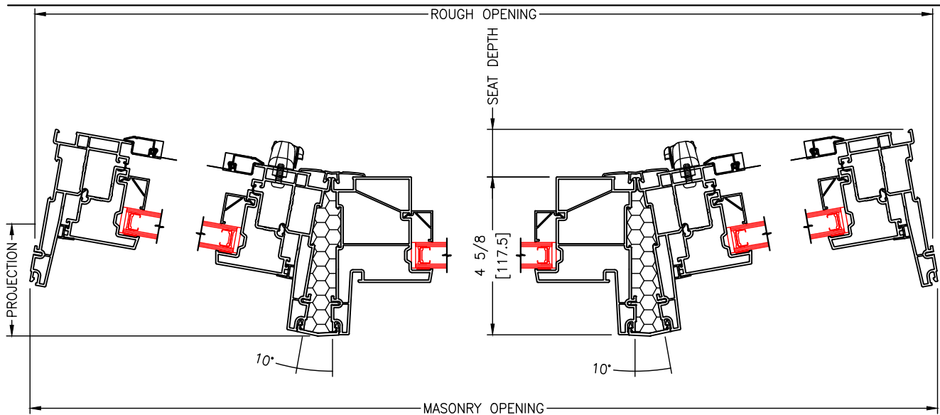
3-WIDE 10° BOW WINDOW HORIZONTAL SECTION (SHOWN)
