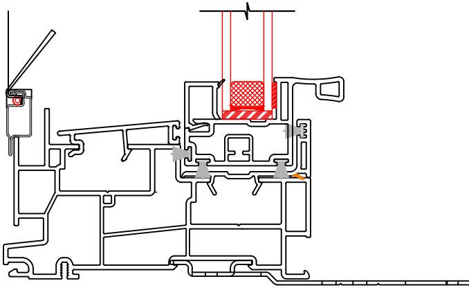
MASONRY CLIP
