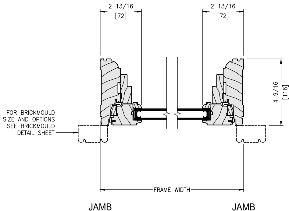
HORIZONTAL SECTION
