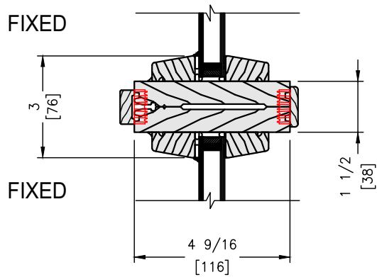
VERTICAL SECTION
