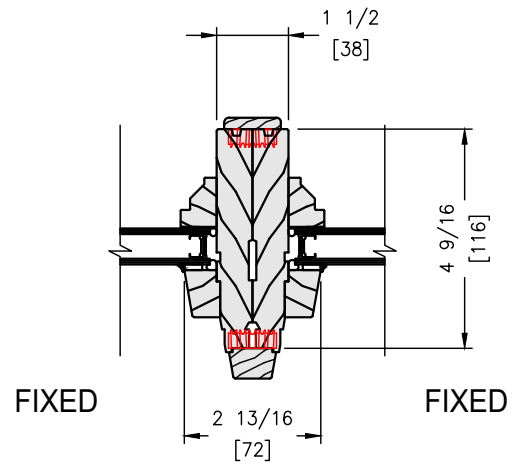
HORIZONTAL SECTION
