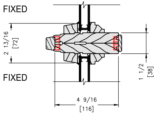
VERTICAL SECTION
