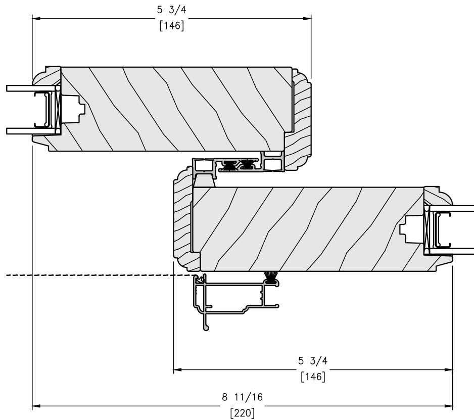
MEETING RAILS
